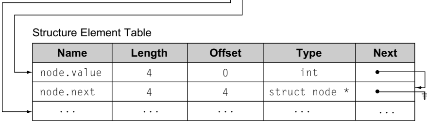
■ FIGURE 7.12 Structure Tables for the List Example.
